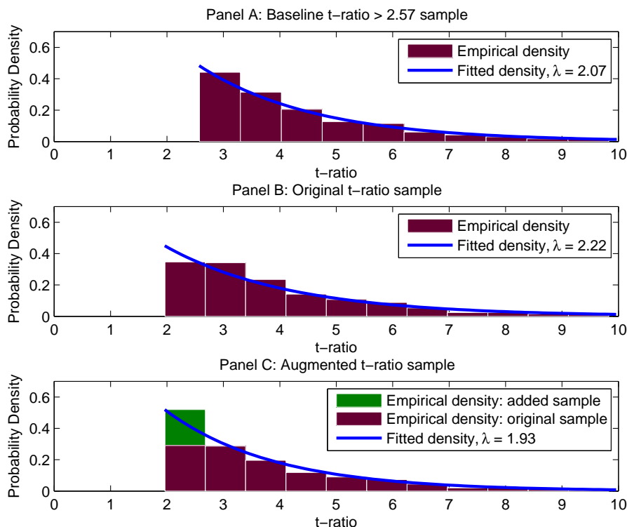
Figure A.1: Density Plots for t-ratio
